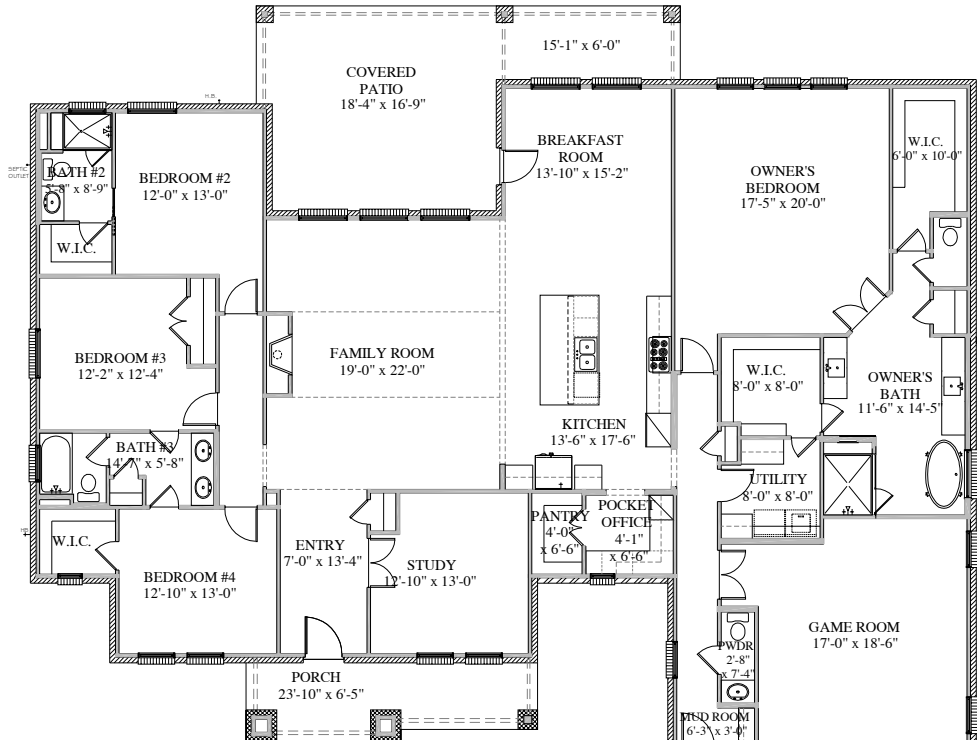
FLOOR PLAN
